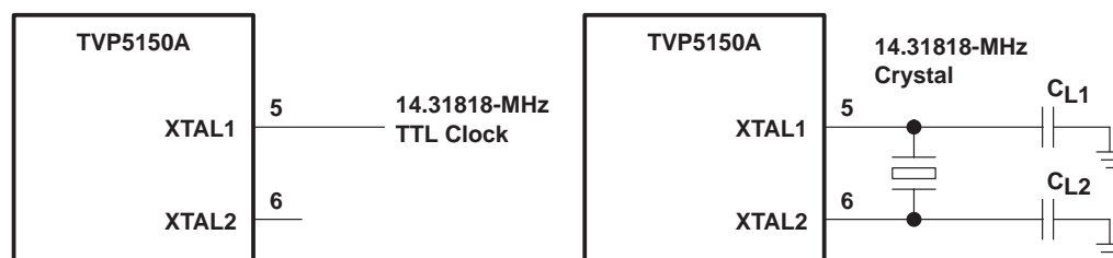
Figure 2–5. Reference Clock Configurations
