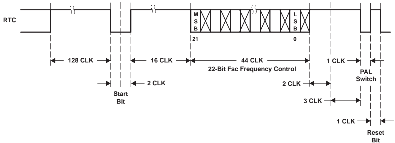
Figure 2–7. RTC Timing
