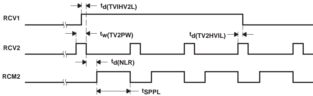
Figure 3–2. Demand Mode Timing
