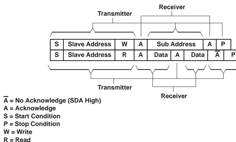
Figure 2–5. I 2 C Read Cycle
