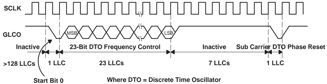
Figure 2–14. Transmission Timing
