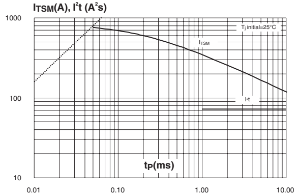
Figure 8: Non repetitive surge peak on-state current for a sinusoidal pulse with width t_p < 10\text{ms} , and corresponding value of I^2t
