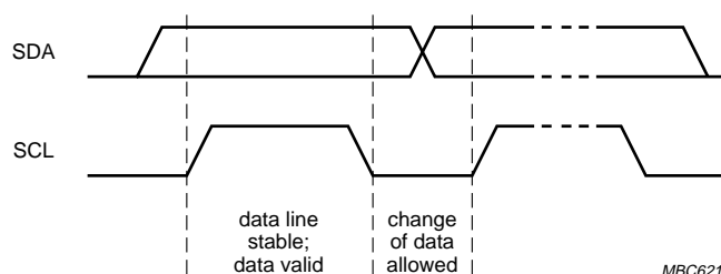
Fig.11 Bit transfer.
