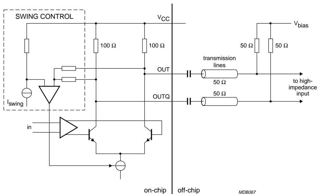
Fig.25 Parallel output CML mode (AC-coupled).
