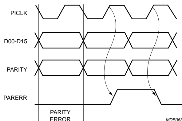
Fig.9 Parity timing.
