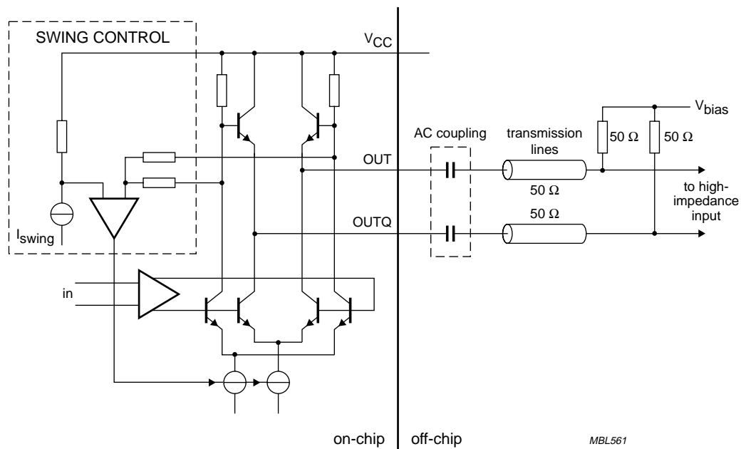
Fig.24 Parallel output floating LVPECL mode (AC-coupled).
