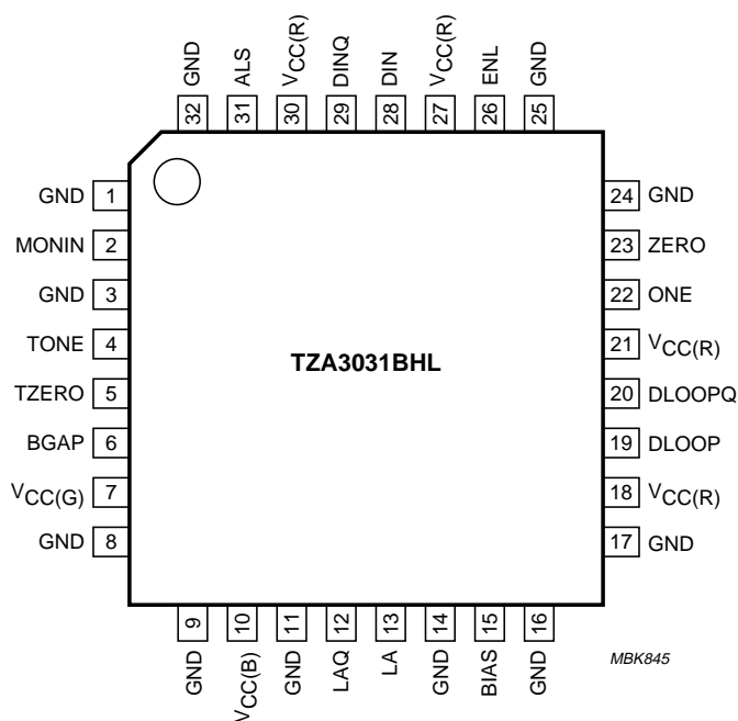
Fig.4 Pin configuration of TZA3031BHL.
