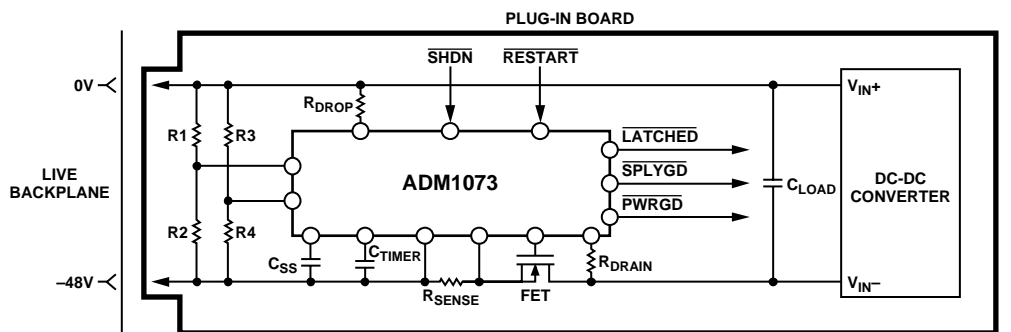
Figure 31. ADM1073 Topology
