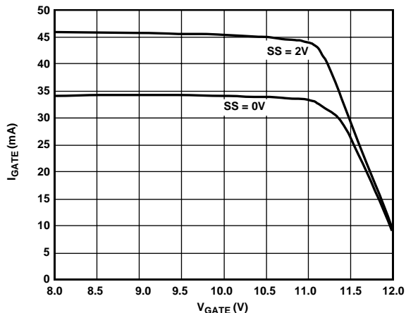
Figure 12. I_{GATE} (Source) vs. V_{GATE}
