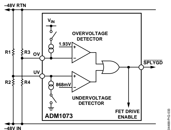
Figure 33. Undervoltage and Overvoltage Circuitry (Standard 4-Resistor Configuration)
