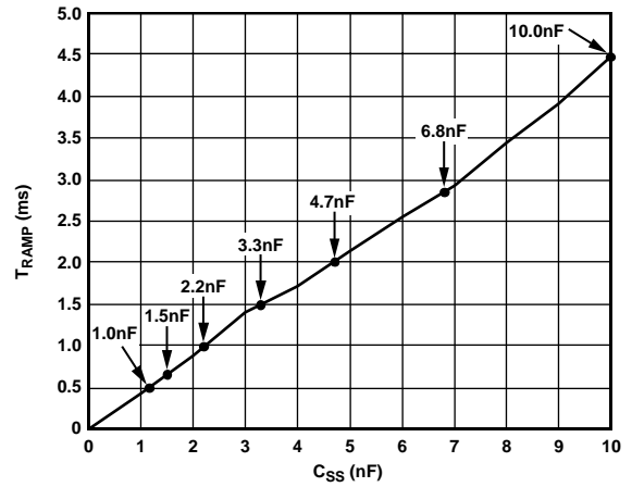
Figure 29. Soft Start Ramp Time vs. C SS
