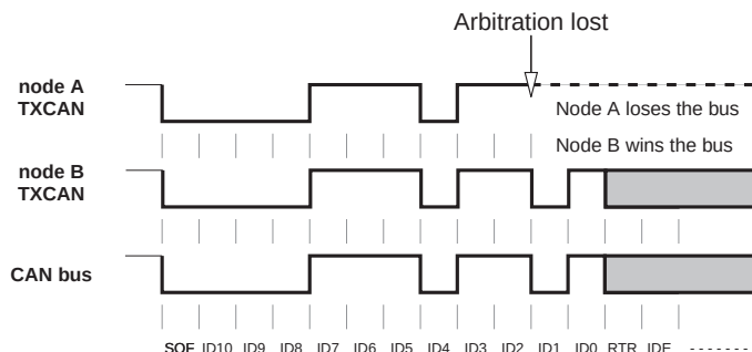
Figure 46. Bus Arbitration
