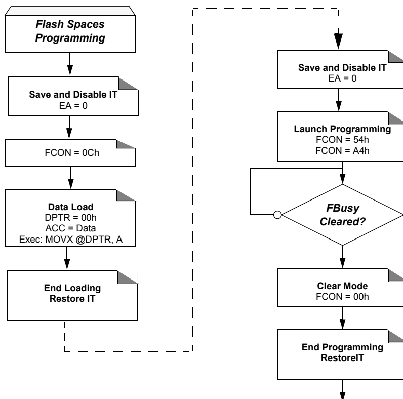
Figure 27. Hardware Programming Procedure
