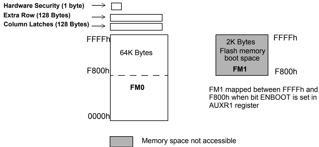
Figure 24. Flash Memory Architecture with ENBOOT=0 (user mode)
