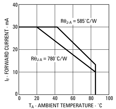
Figure 7. Forward Current vs. Ambient Temperature.
