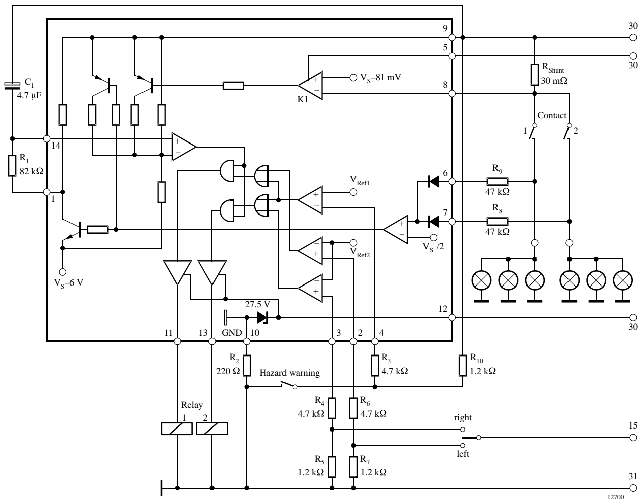
Figure 2. Application circuit
