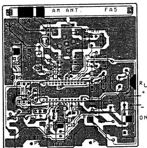
Figure 19. PC-board
