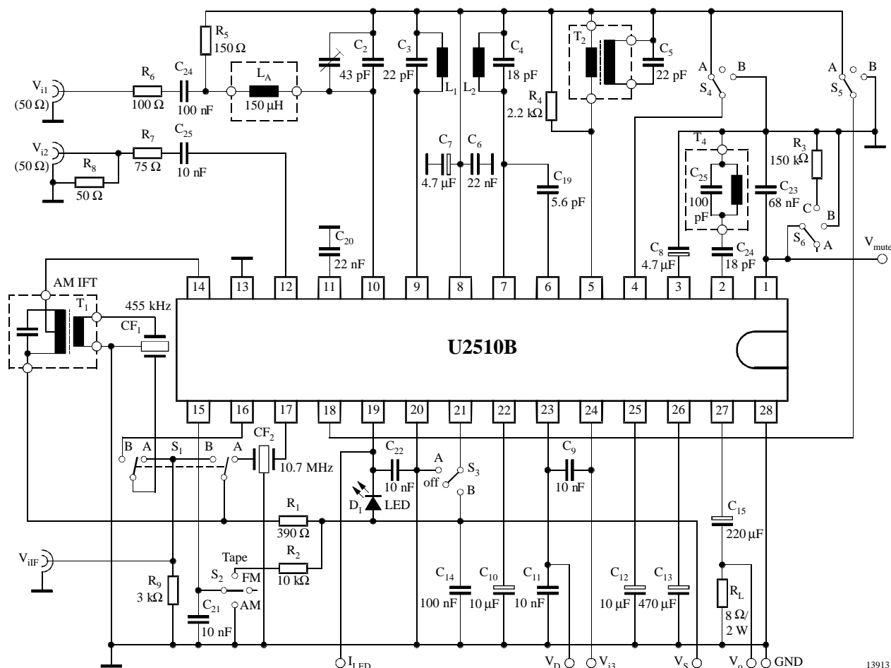
Figure 16. Test circuit
