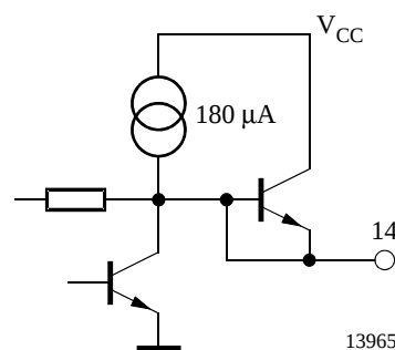
Figure 10. Pin 14: Demodulator output
