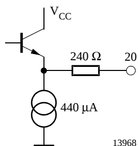
Figure 13. Pin 20: Limiter 1 output
