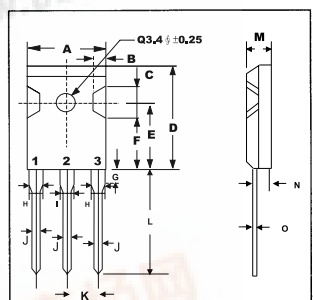
TO-247 (3P)
