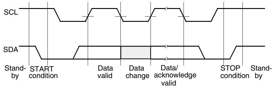
Figure 6. Serial Protocol
