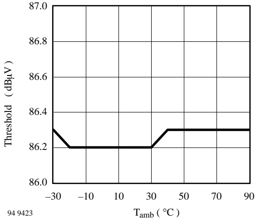
AGC threshold ( I_{I0} = 1 \mu\text{A} ) of the second IF amplifier versus temperature
