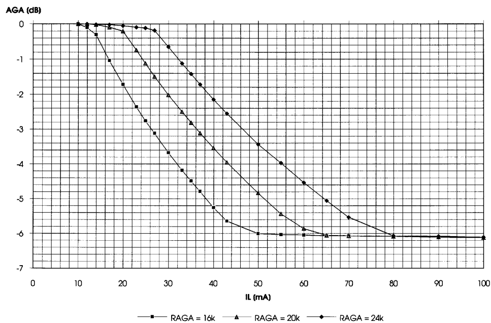
Figure 15. Typical AGA Characteristic
