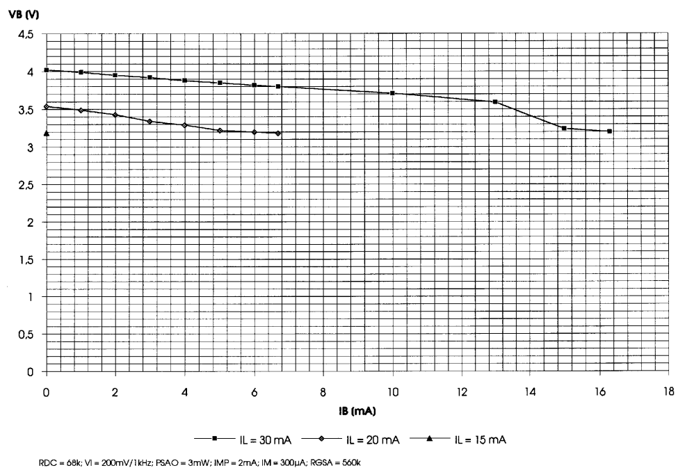
Figure 18. Typical Load Characteristic of V_B for a Minimum DC Characteristic ( R_{DC} = 68\text{ k}\Omega ) and a 3-mW Loudspeaker Output
