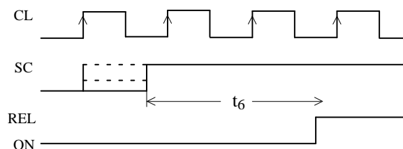
Figure 2. The debouncing of the short circuit detection
