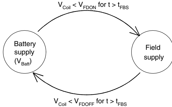
Figure 6. Switch Conditions for Power Management
