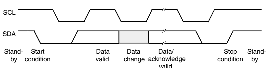
Figure 7. Serial Protocol
