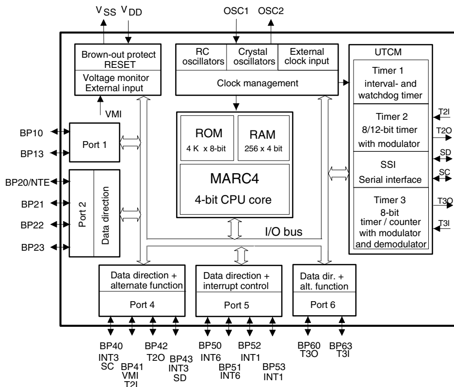
Figure 3. Block Diagram ATAR092
