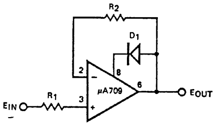
LATCH-UP PROTECTION
