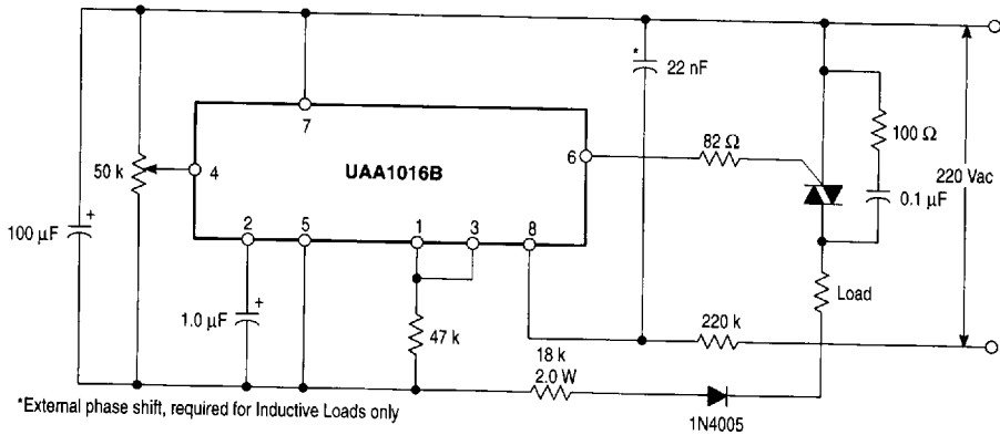
Figure 8. Electronic Rheostat
