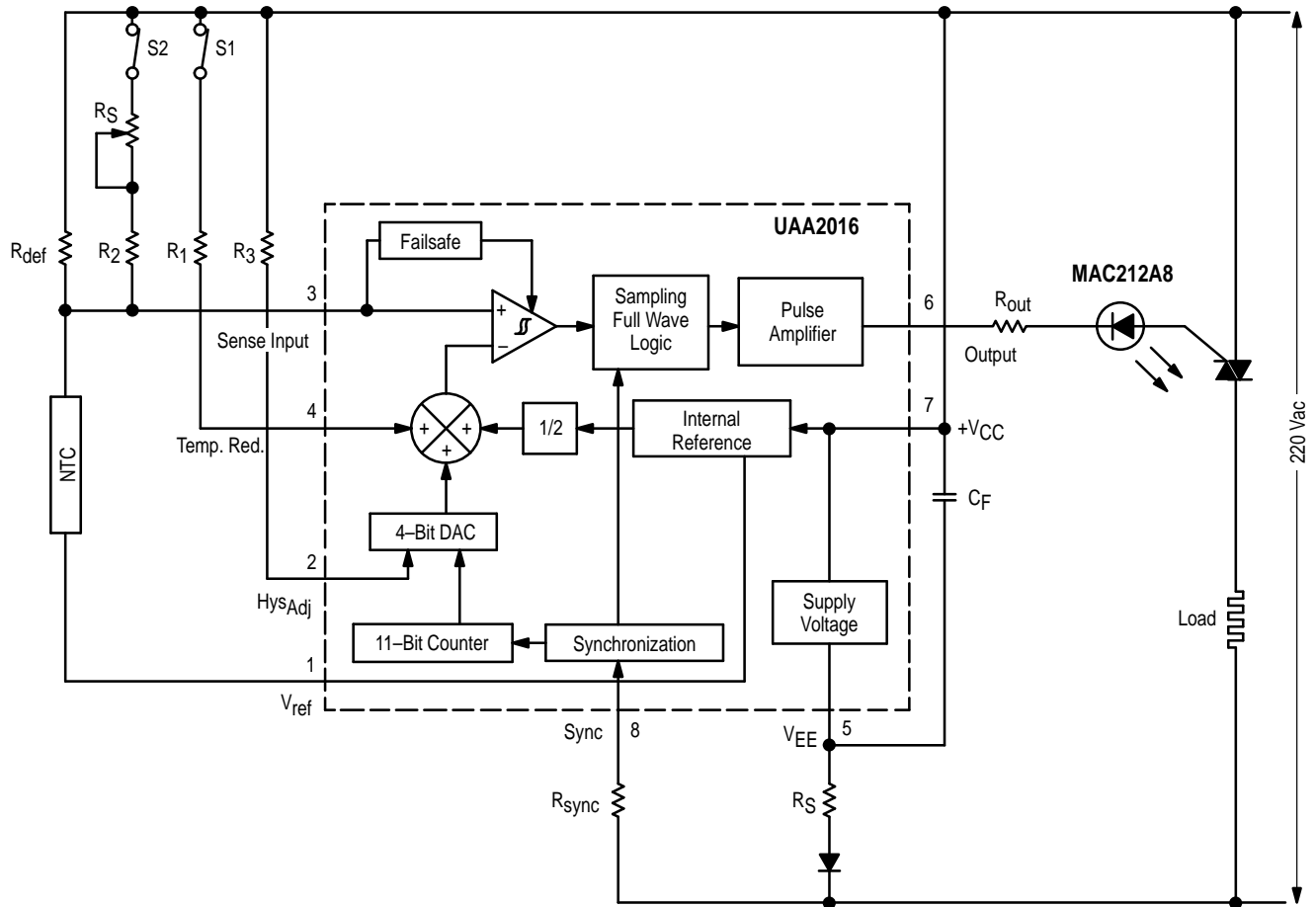
Figure 1. Application Schematic
