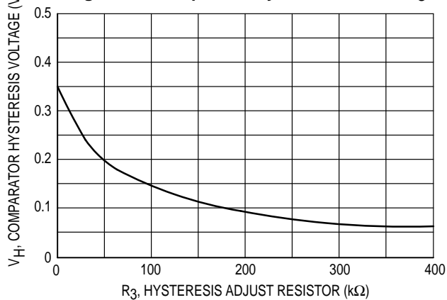
Figure 17. Comparator Hysteresis versus R_3
