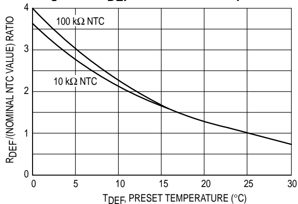
Figure 15. R_{DEF} versus Preset Temperature
