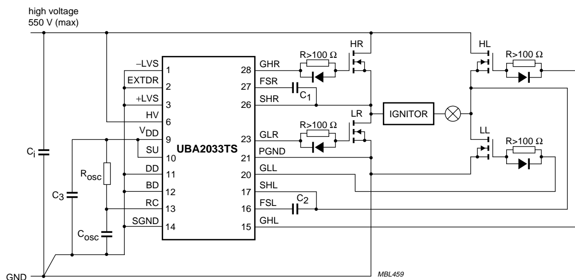
Fig.3 Basic configuration.
