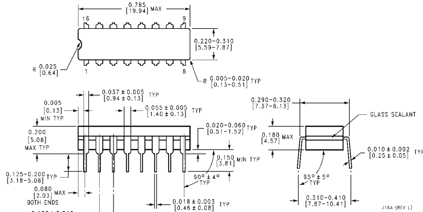
Ceramic Dual-In-Line Package (J) Order Number CD4049UBMJ, CD4049UBCJ, CD4049BMJ or CD4049BCJ NS Package Number J16A
