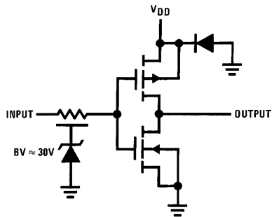
CD4049UBM/CD4049UBC 1 of 6 Identical Units
