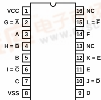
CD4049UBMS TOP VIEW
