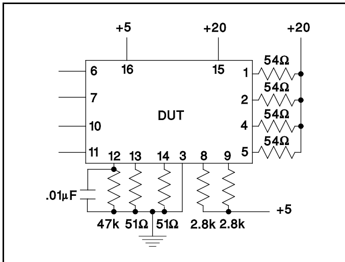
Figure 3. Test Circuit
