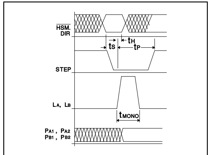
Figure 4. Timing Waveforms
