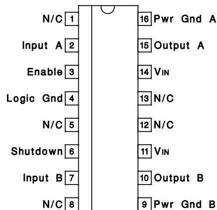
SOIC-16 (Top View) DW Package
