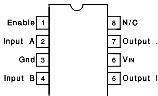
DIL-8 (Top View) J Or N Package
