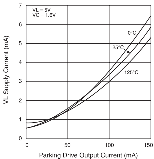
VL Current vs. PRKDRV Current
