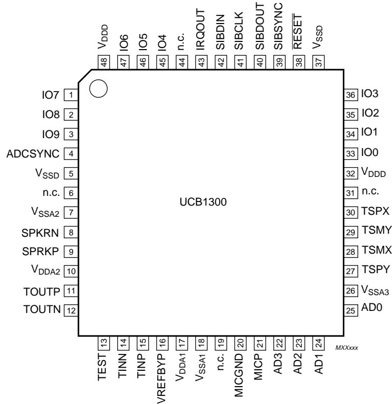
Fig.2 Pin configuration.
