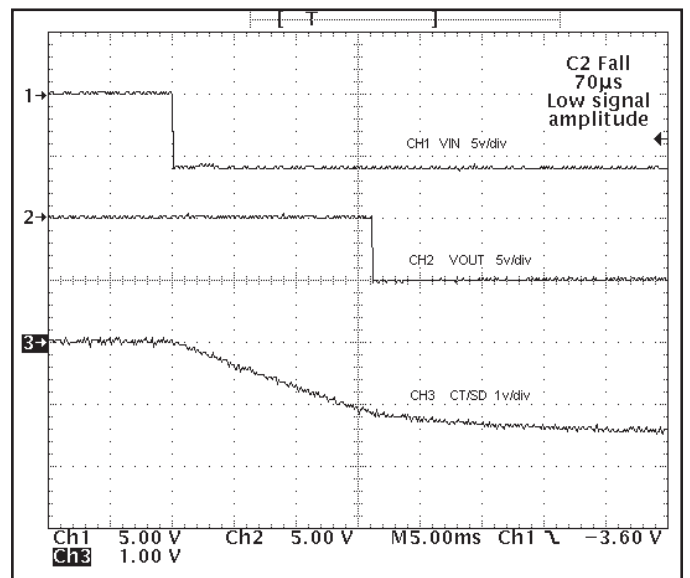
Figure 10. VIN to VOUT delay time during power-up with CT = 0.22 µF
