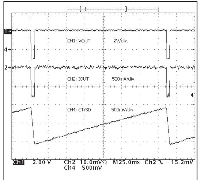
Figure 7. UCC384-ADJ operation during overcurrent condition (25ms/div.).
