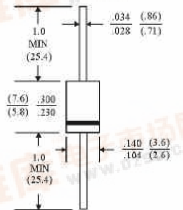
DO-15
