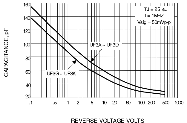
Fig. 6-TYPICAL JUNCTION CAPACITANCE
