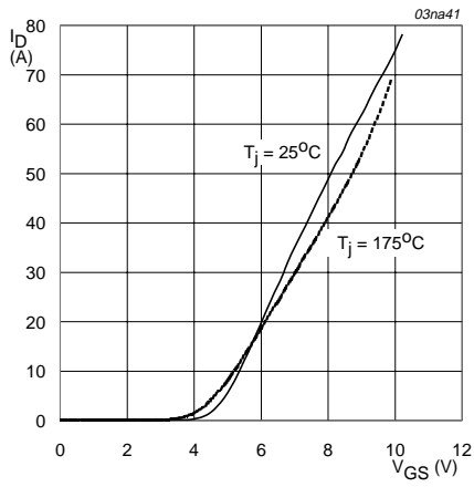
Fig 13. Transfer characteristics; typical values.
