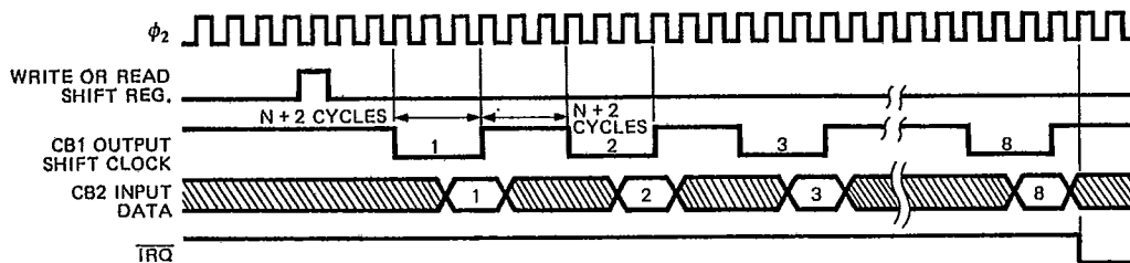
Figure 23-1 Shift Register Input Modes 5-31
