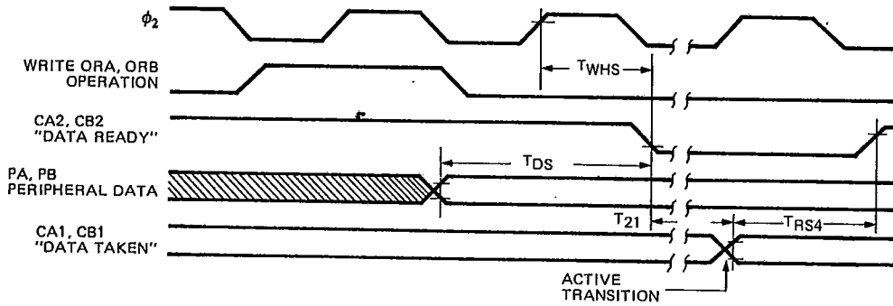
Figure 5d. CA2, CB2 Timing for Write Handshake, Handshake Mode
