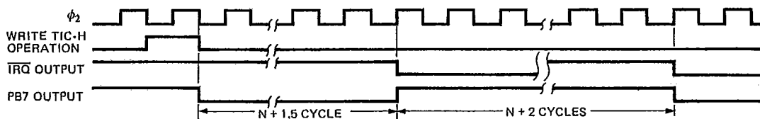
Figure 19. Timer 1 Free-Run Mode Timing
