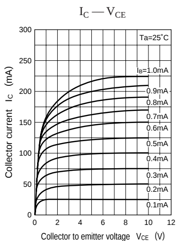
Characteristics charts of UN1222
