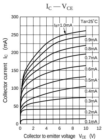
Characteristics charts of UN1221
