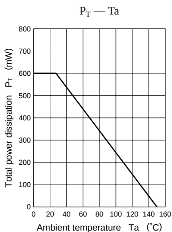
Characteristics charts of UN1221
