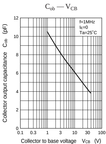
Characteristics charts of UN1223
