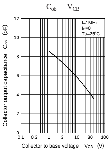
Characteristics charts of UN1224
