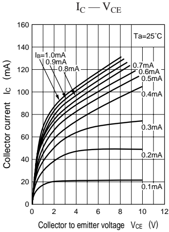
Characteristics charts of UN4212
