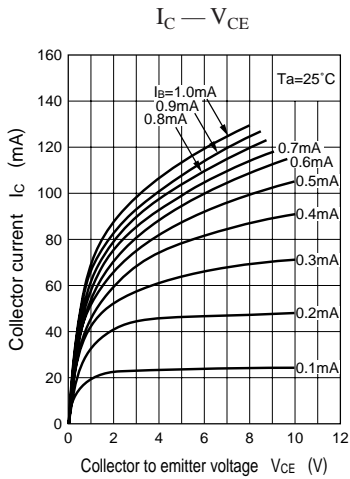
Characteristics charts of UN4215
