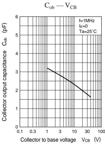
Characteristics charts of UN4216
