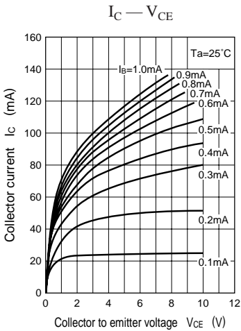
Characteristics charts of UN4213
