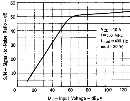
SIGNAL-TO-NOISE RATIO
