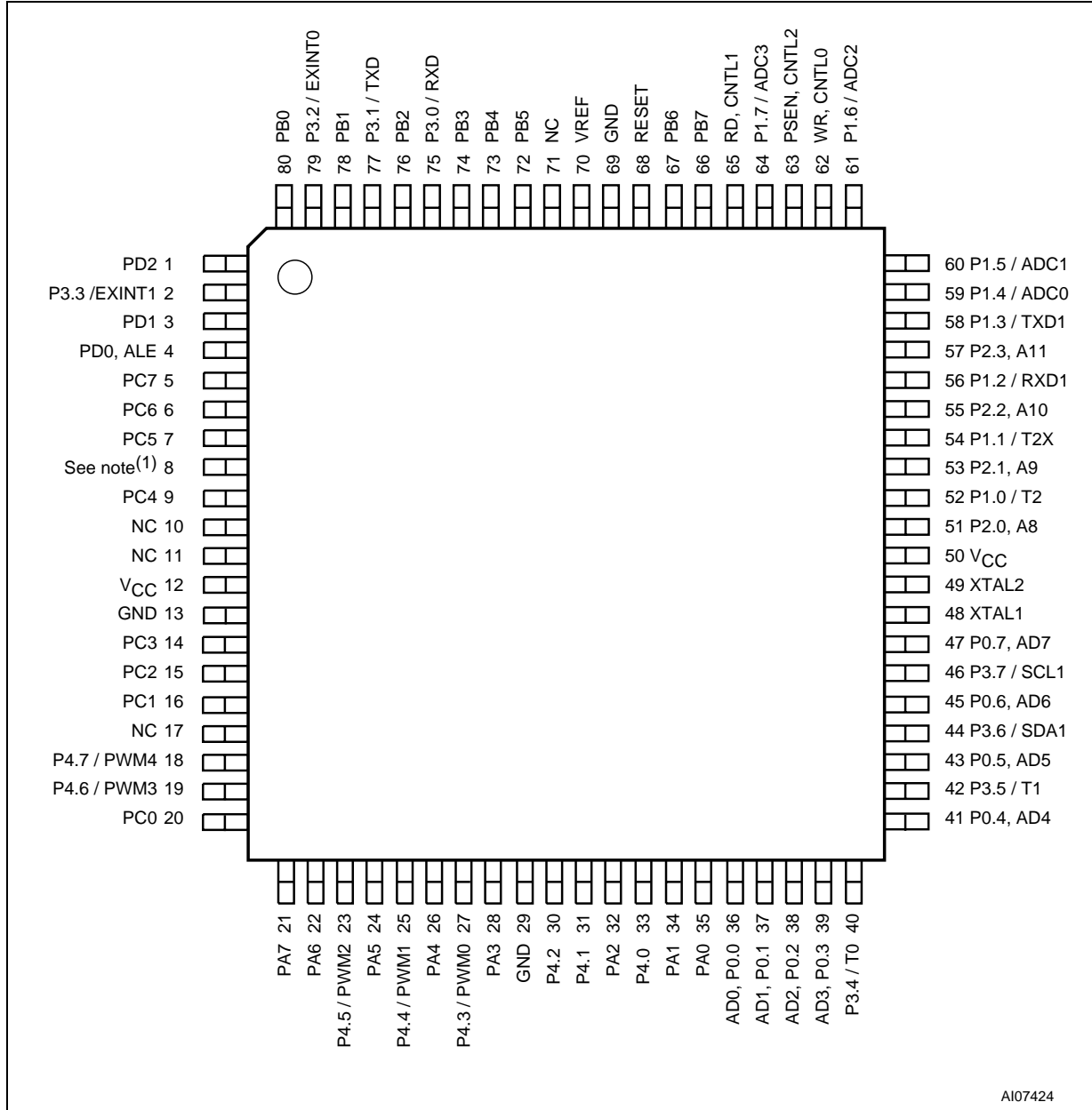
Figure 4. TQFP80 Connections
