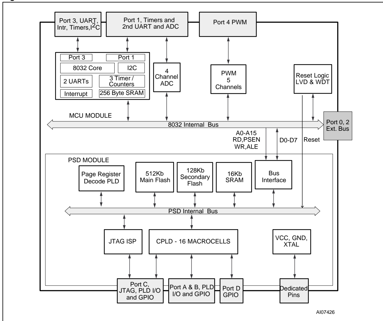
Figure 15. uPSD321X Devices Functional Modules
