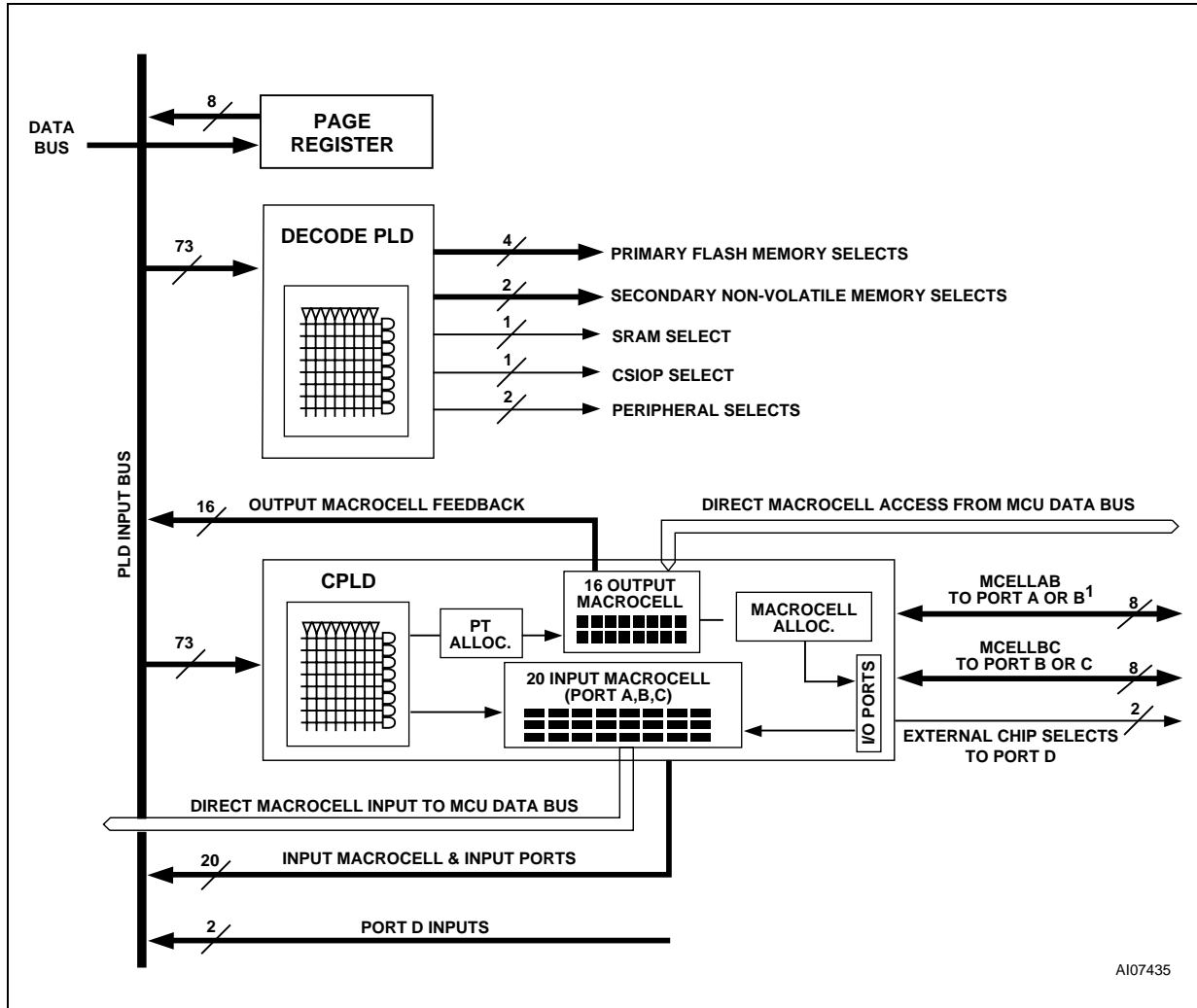
Figure 48. PLD Diagram
