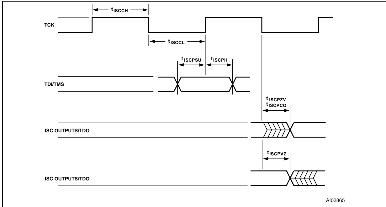
Figure 76. ISC Timing
