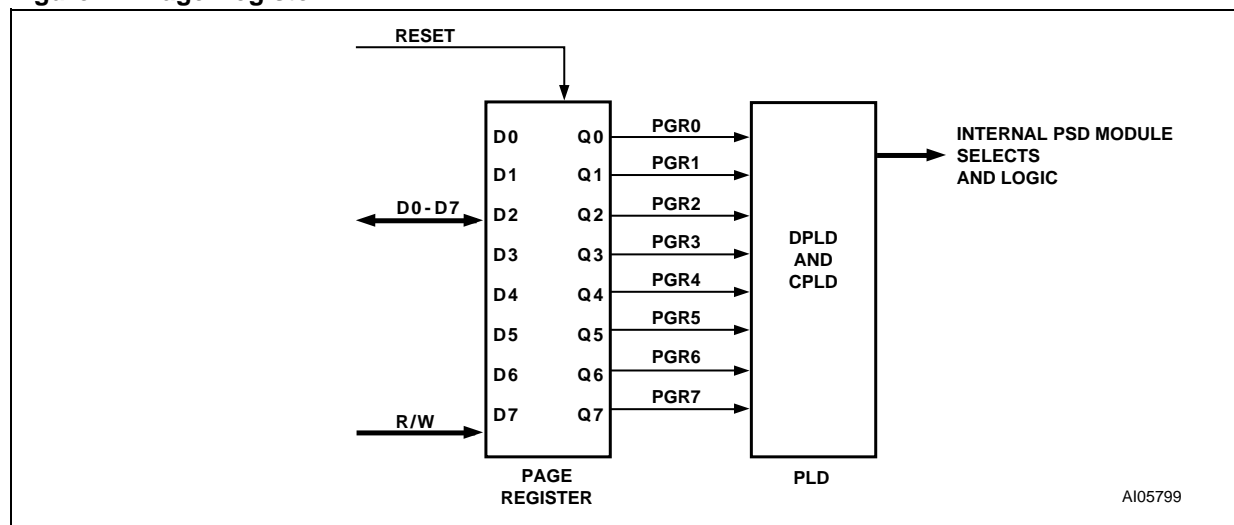
Figure 47. Page Register
