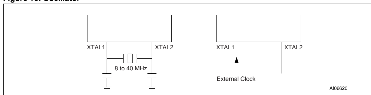
Figure 19. Oscillator
