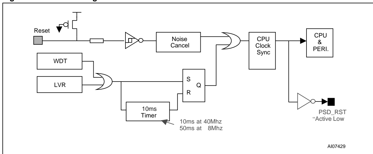
Figure 20. \overline{\text{RESET}} Configuration
