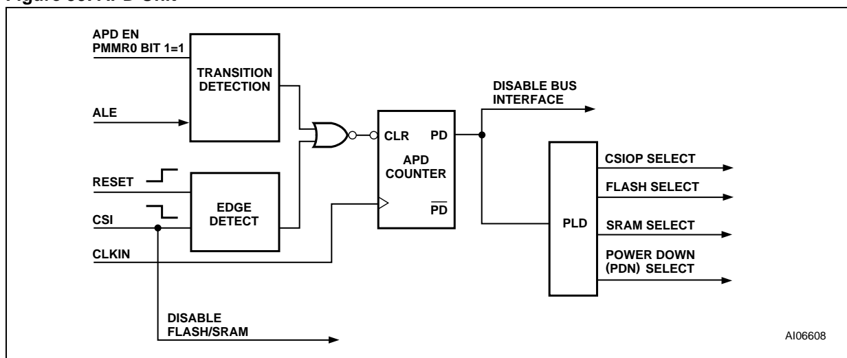
Figure 59. APD Unit
