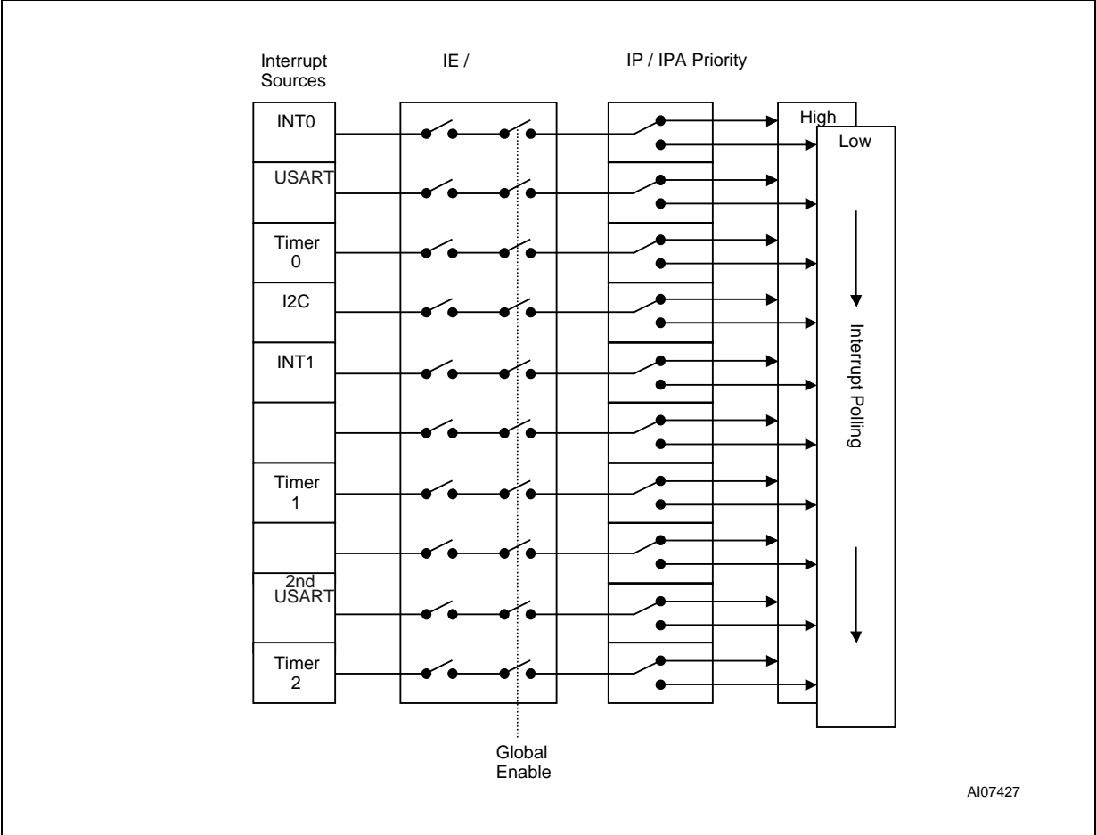
Figure 16. Interrupt System
