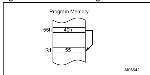
Figure 12. Indirect Addressing
