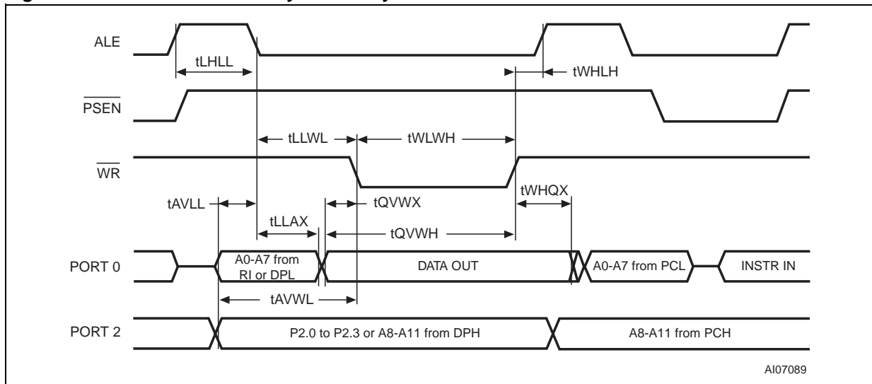
Figure 67. External Data Memory WRITE Cycle
