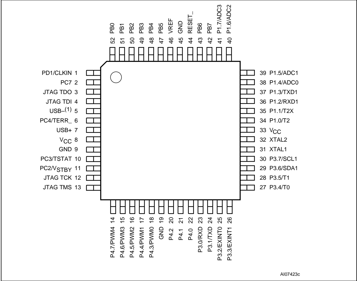
Figure 3. TQFP52 Connections
