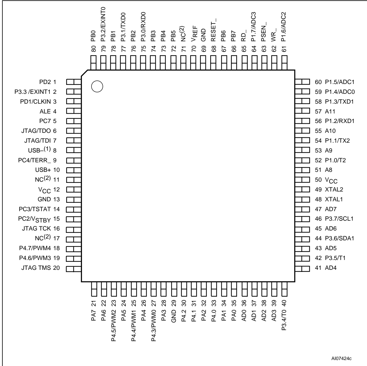
Figure 4. TQFP80 Connections
