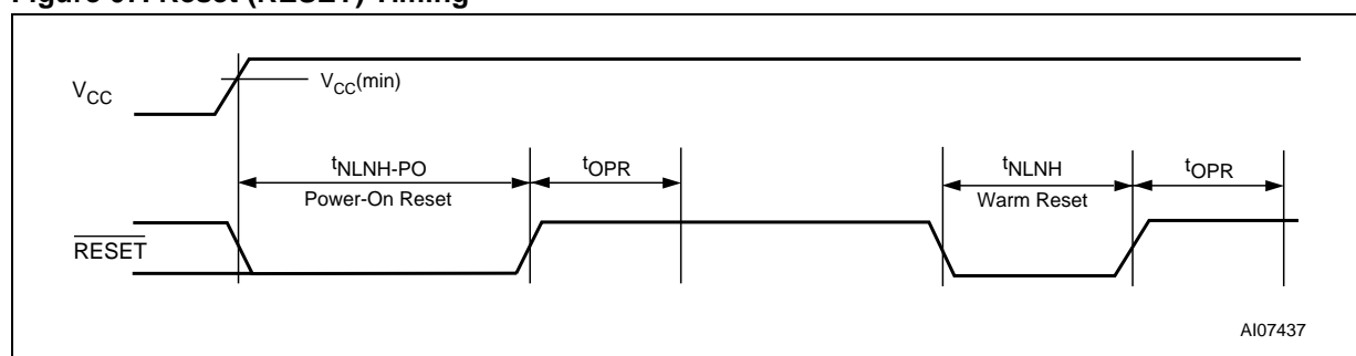
Figure 67. Reset ( \overline{\text{RESET}} ) Timing
