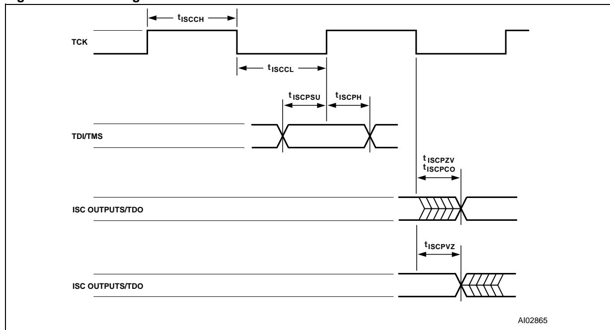
Figure 82. ISC Timing
