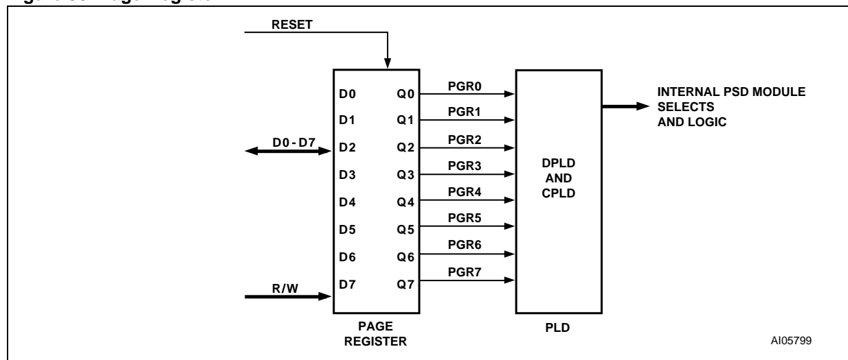
Figure 53. Page Register
