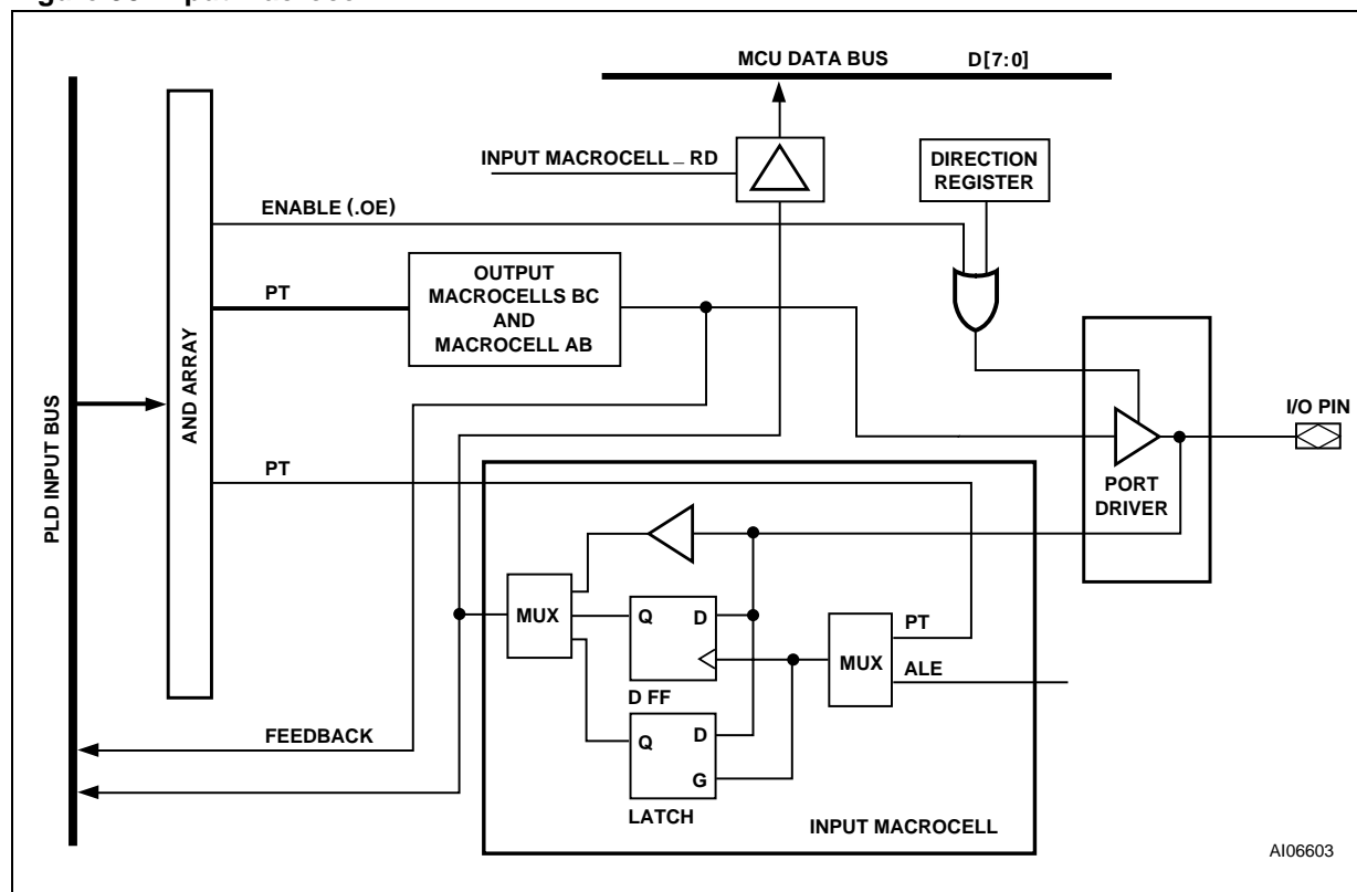
Figure 58. Input Macrocell
