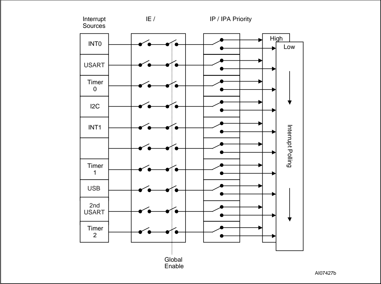
Figure 16. Interrupt System
