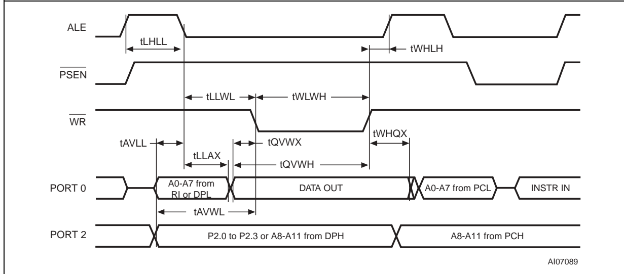
Figure 73. External Data Memory WRITE Cycle
