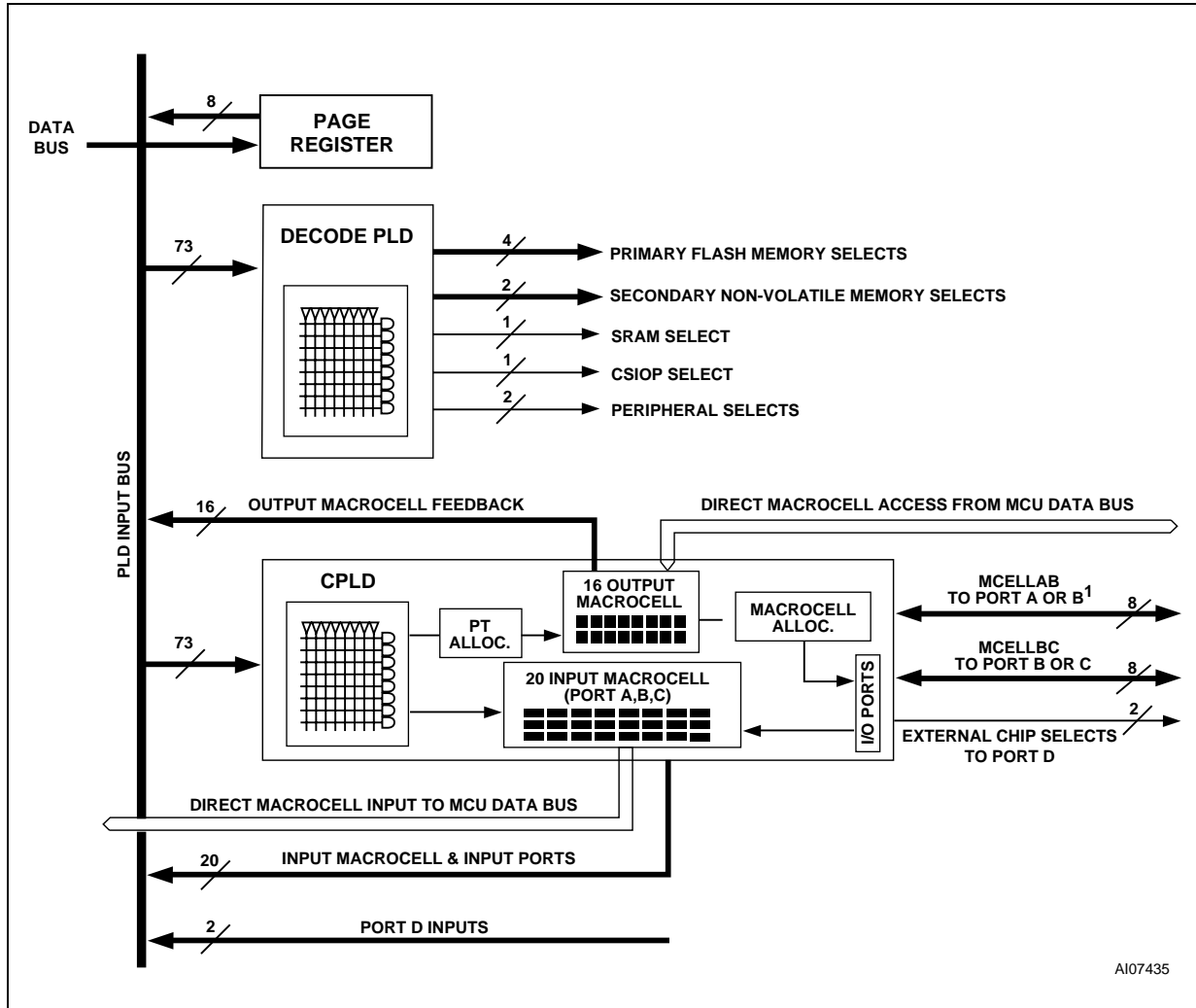
Figure 54. PLD Diagram
