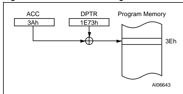
Figure 13. Indexed Addressing
