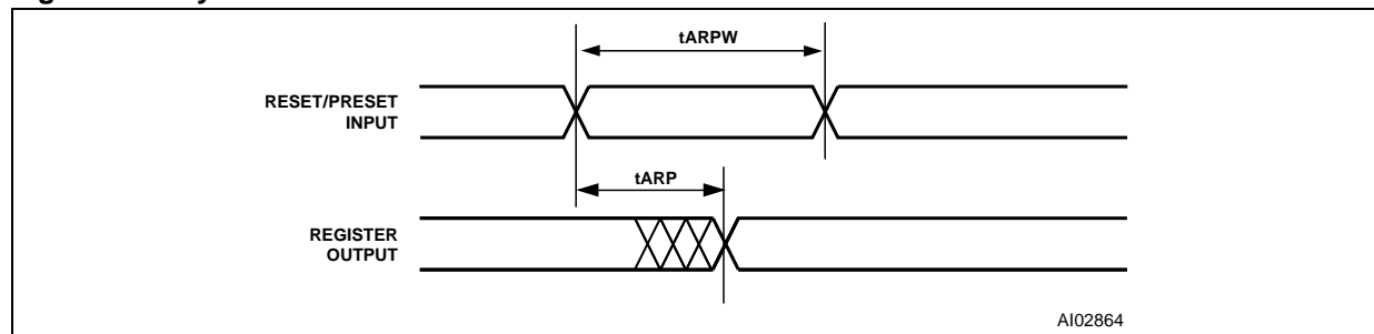
Figure 76. Asynchronous \overline{RESET} / Preset
