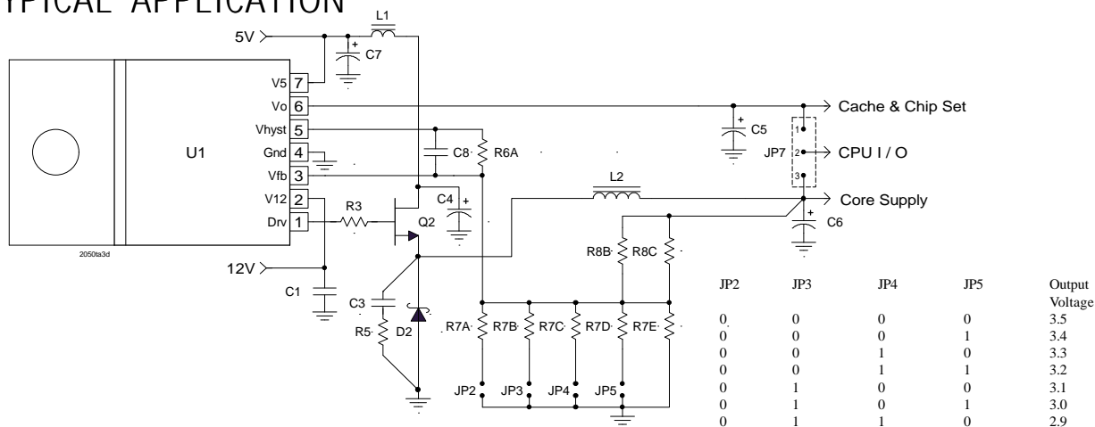
Figure2- Typical application of US2075 in a flexible motherboard with the 4 bit VID output voltage selection. This circuit uses a single jumper that programs the output voltage in 16 steps with 0.1V steps from 2V to 3.5V, designed for Intel P55™, P54™, AMD K5 & K6™ as well as Cyrix M1™ and M2™ applications. The jumper JP7 selects between single supply and dual supply processors.
