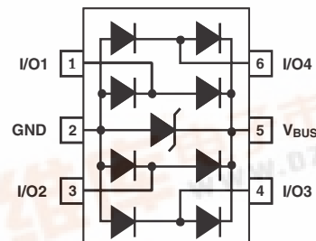
Figure 1: Functional Diagram
