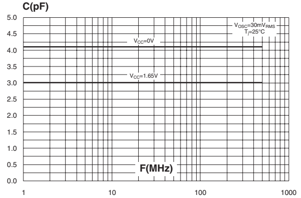
Figure 5: Frequency response
