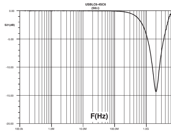
Figure 5: Frequency response
