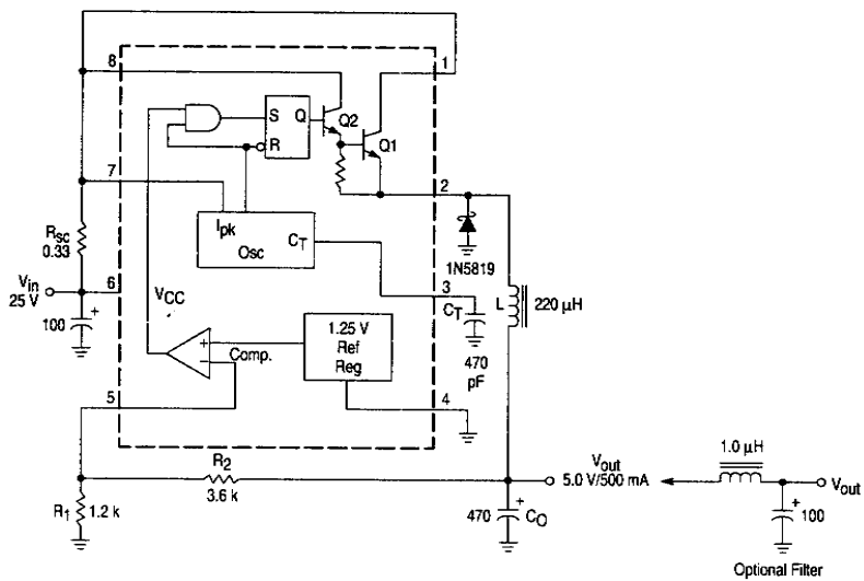
Figure 9. Step-Down Converter
