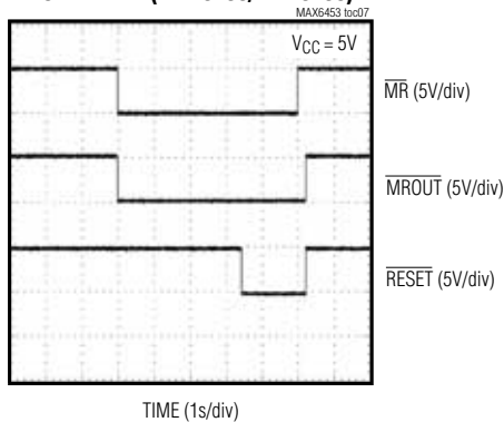
MANUAL RESET TO \overline{\text{MROUT}} AND RESET DELAY (MAX6455/MAX6456)
