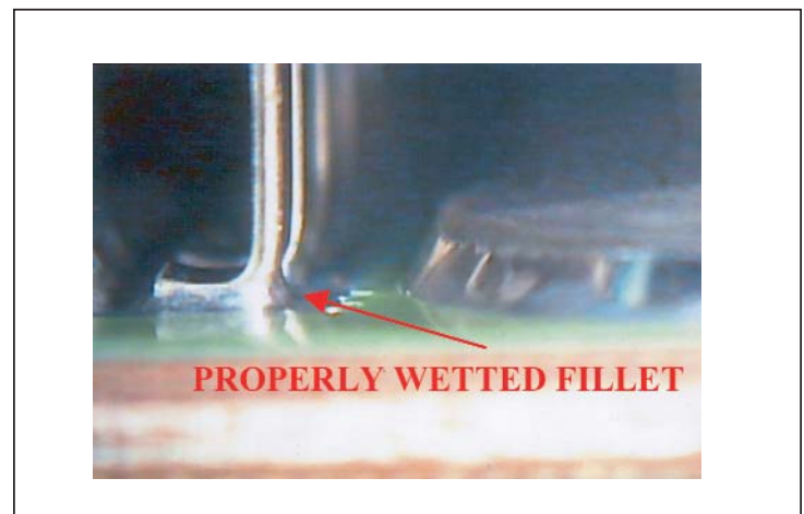
Figure 26— Properly reflowed V•I Chip J-Lead.
