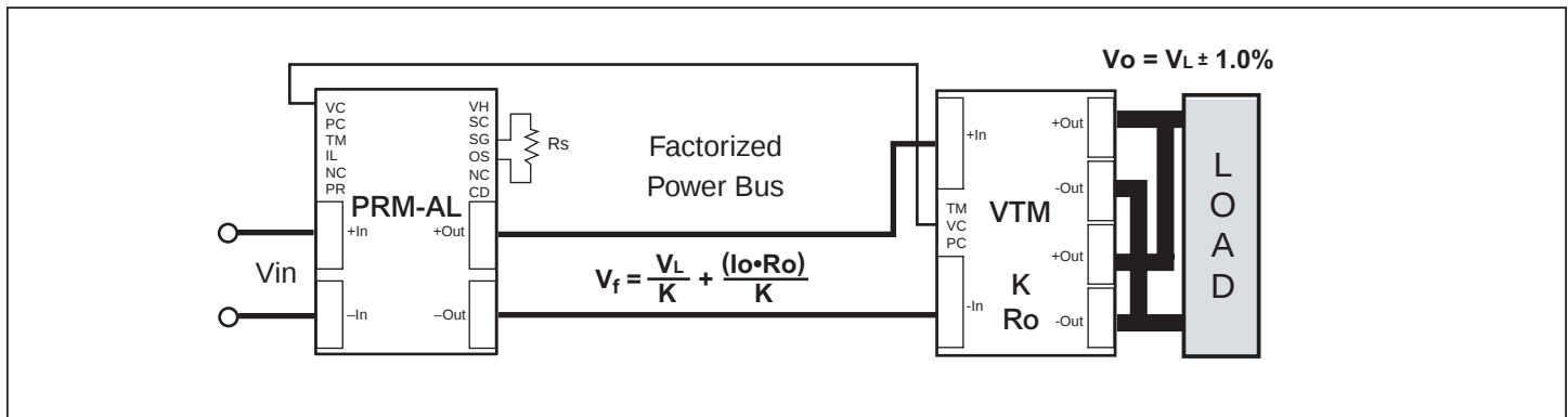
Figure 21 — The PRM controls the factorized bus voltage, Vf, in proportion to output current to compensate for the output resistance, Ro, of the VTM. The VTM output voltage is typically within 1% of the desired load voltage (VL) over all line and load conditions.
