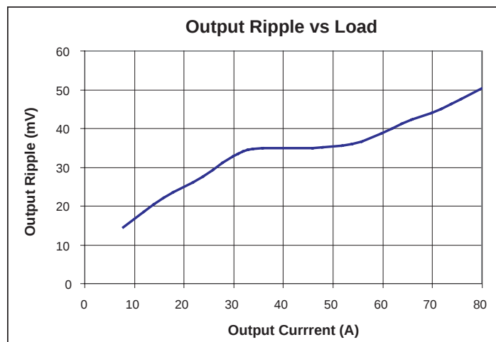
Figure 2— Output voltage ripple vs. output current at 2 Vout with no POL bypass capacitance.
