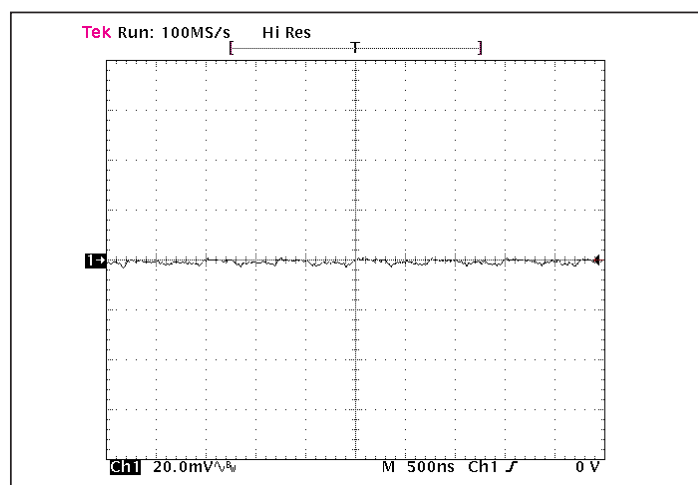
Figure 6— Output voltage ripple at full load and 2 Vout with 100 \mu F ceramic external bypass capacitance and 20 nH distribution inductance.
