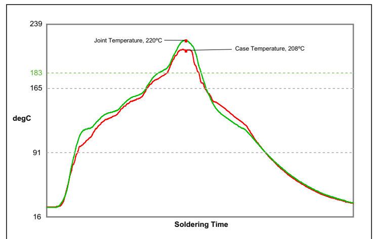
Figure 25—Thermal profile diagram
