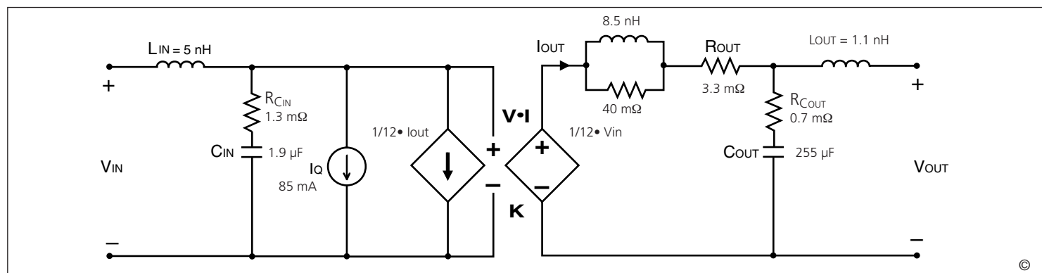
Figure 18 —This model characterizes the AC operation of the V•I Chip VTM including response to output load or input voltage transients or steady state modulations. The model enables estimates or simulations of input and output voltages under transient conditions, including response to a stepped load with or without external filtering elements.
