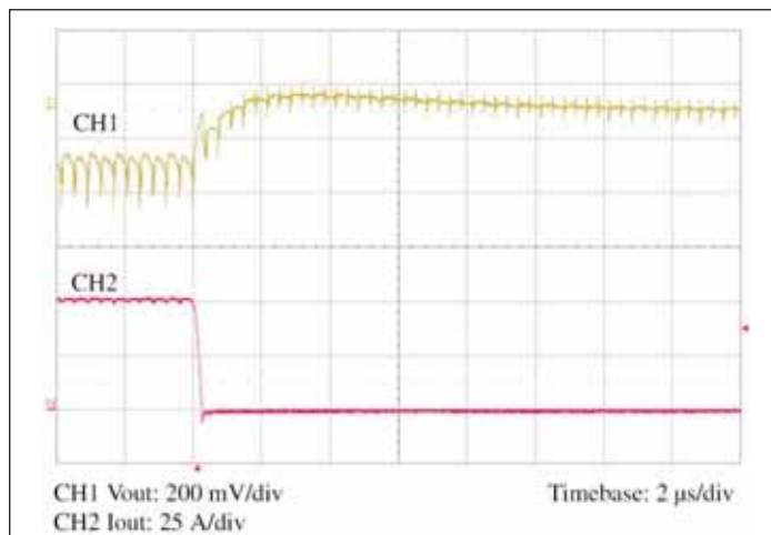
Figure 8 — 50-0 A load step with 100 \mu F input capacitance and no output capacitance.
