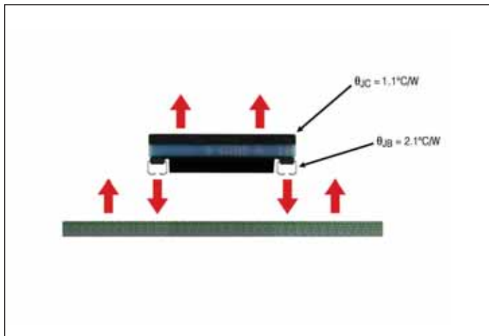
Figure 15 —Thermal resistance
