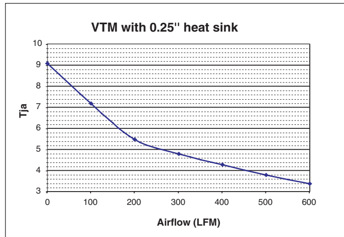
Figure 16 —Junction-to-ambient thermal resistance of VTM with 0.25" Heat Sink.
