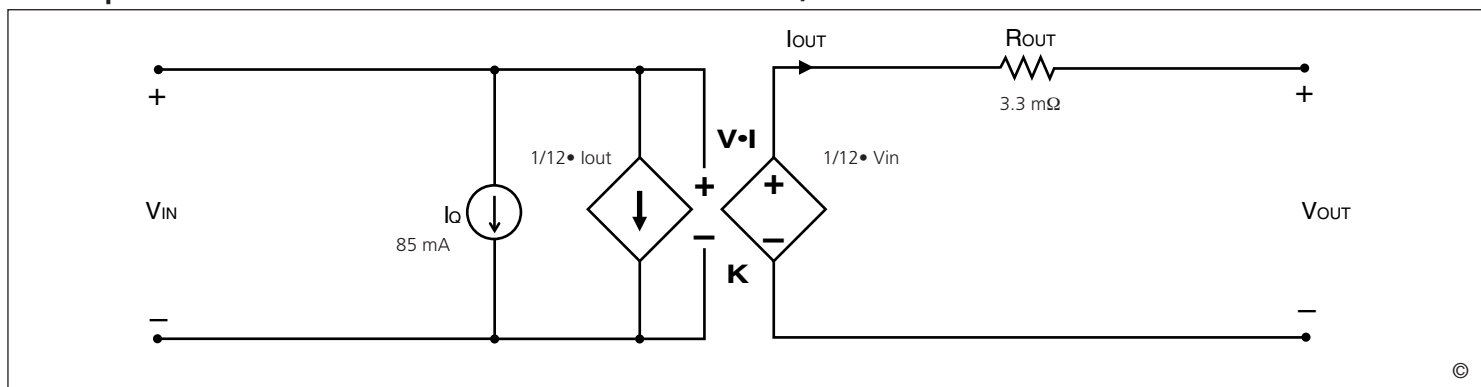
Figure 17 —This model characterizes the DC operation of the V•I Chip VTM, including the converter transfer function and its losses. The model enables estimates or simulations of output voltage as a function of input voltage and output load, as well as total converter power dissipation or heat generation.
