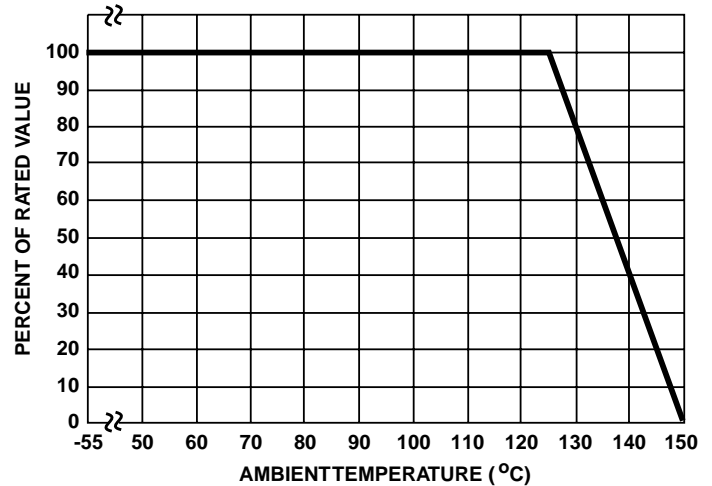
FIGURE 1. CURRENT, ENERGY AND POWER DERATING CURVE
