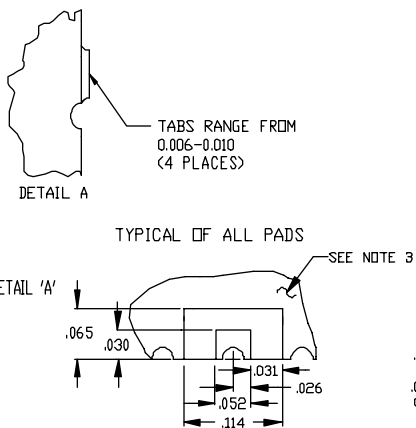
PHYSICAL DIMENSIONS
