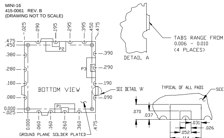
PHYSICAL DIMENSIONS
