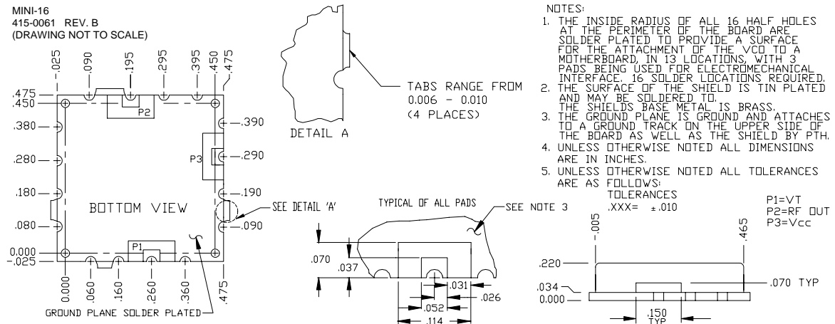
PHYSICAL DIMENSIONS
