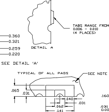
PHYSICAL DIMENSIONS
