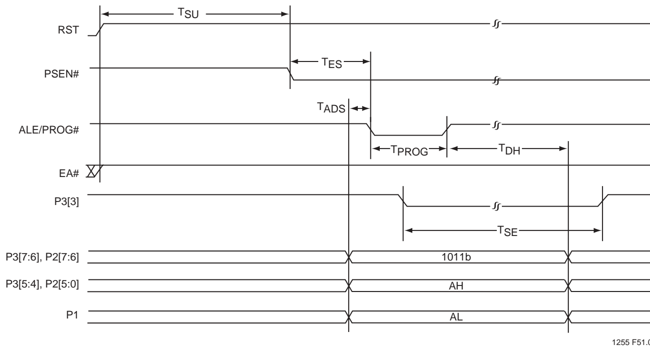
FIGURE 14-19: SECTOR-ERASE
