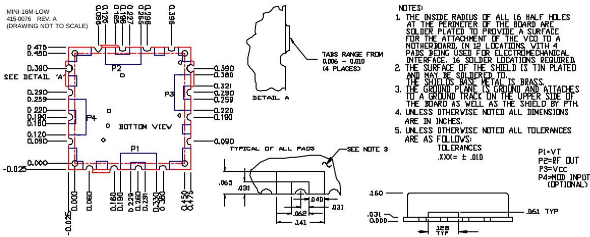
PHYSICAL DIMENSIONS
